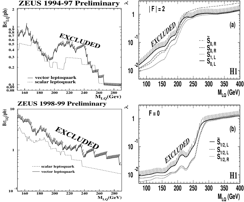
Figure 6. ZEUS limits at 95% C.L. on \sigma \cdot \beta for scalar (dotted lines) and vector \lambda = \lambda_{1j} for different scalar LQ's with (full lines) LQ's, from the e^+p [11] (top) |F|=2 (top) and F=0 (bottom). Only and the e^-p [13] (bottom) data. NC-type data are used for these limits.
