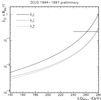
Figure 10. ZEUS exclusion limits at 95% C.L. on \lambda_{1j} \cdot \text{BR}(LQ \rightarrow \mu q) for three types of scalar LQ's coupling to electrons and muons and to d , u , and d and u quarks, respectively (top to bottom). The horizontal line indicates electromagnetic coupling strength.
