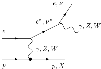
Figure 1. Feynman graph of the production and subsequent decay of excited electrons or neutrinos in ep reactions. Note that alternatively also an excited quark could be produced at the boson-proton vertex. In the case of e^* production, elastic reactions ep \rightarrow e^*p are possible.
