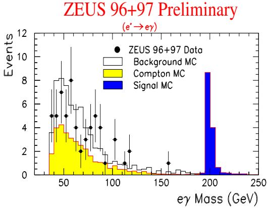
Figure 2. Spectrum of the invariant e\gamma mass of ZEUS candidates for e^* production and subsequent decay e^* \rightarrow e\gamma . The points with error bars represent the data, the open (light-shaded) histogram the total SM background (the contribution from QED Compton scattering). The dark-shaded histogram illustrates the signal expected for a hypothetical e^* with a mass of 200 GeV.
