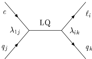
Figure 4. Feynman graph of the resonant production of a F=2 LQ in electron-quark scattering. The subscripts of the Yukawa couplings at production and decay vertex of the LQ indicate the generations of the leptons and quarks involved.
