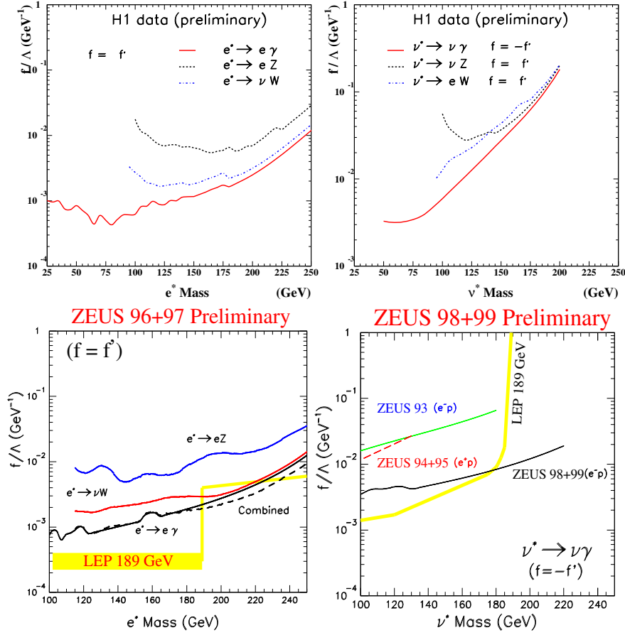
Figure 3. Limits at 95% C.L. on f/\Lambda from H1 (top) and ZEUS (bottom) searches for excited electrons (left) and excited neutrinos (right). The shaded bands denoted “LEP 189 GeV” indicate the exclusion limits from [5], with the band width approximating the amplitude of their small-scale variations.
