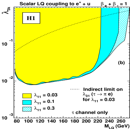
Figure 9. H1 exclusion limits at 95% C.L. on \lambda_{3k} for different fixed values of \lambda_{1j} . Scalar LQ's which only couple to e and \tau ( \beta_e + \beta_\tau = 1 ) are assumed. Also indicated is an indirect limit derived from the non-observation of the lepton-flavor violating decay \tau \rightarrow e\pi .
