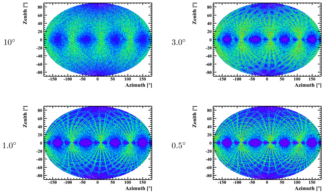
Figure 5.3: Histograms of simulations for pancake-like signals. The displayed information is the same as in the left column of figure 5.1, except for the detector geometry used, which in this case is the ANTARES geometry. The colors show the maximum amplitude received by any hydrophone, each plot for a different pancake opening angle \Phi from 0.5^\circ to 10^\circ .
