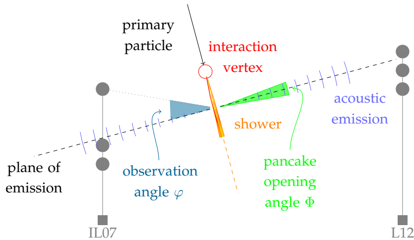
Figure 4.1: Overview of the geometry of acoustic emission from showers. An acoustic pancake-shaped emission (“pancake”) originates from the shower caused by a primary particle. The acoustic emission is rotationally symmetric around the shower axis. The drawing is not to scale.
