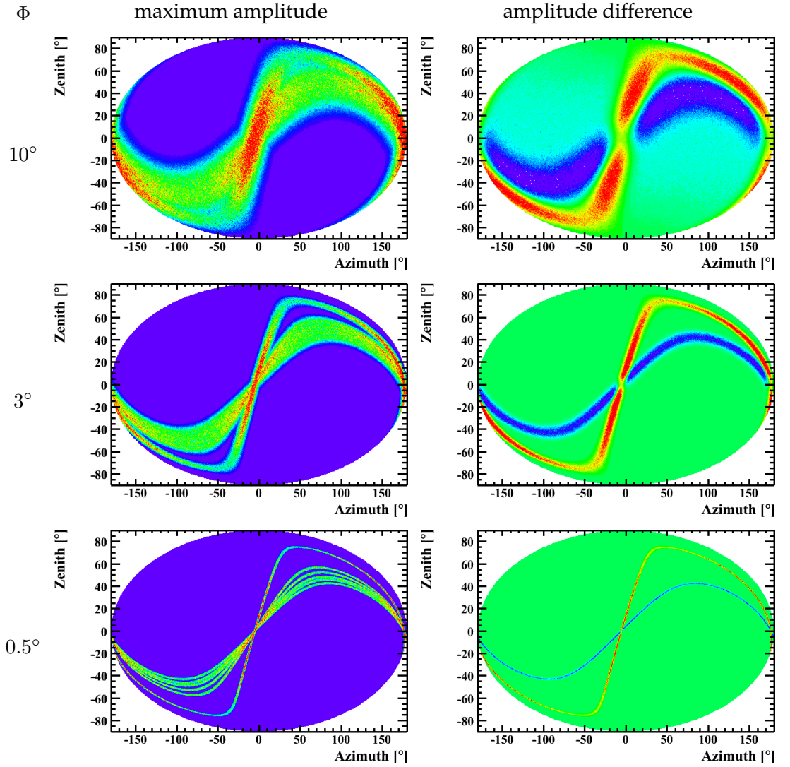
Figure 5.1: Histograms of simulations for pancake-like signals. Azimuth and Zenith values show the direction of the primary particle which caused the signal. The left column shows the maximum amplitude registered by any hydrophone. Blue shows a smaller, red a greater amplitude. Since the plots are only meant to show the spatial distribution, the scale is chosen for best visibility of the features of the plots. The right column shows the difference between two hydrophones OM(1,1) and OM(1,13) from IL07 on the lower- and topmost storey which gives a best-case estimate for the probability to recognize a pancake-like signal and distinguish it from a spherical signal. Green shows a difference of about 0, this corresponds to no ability to distinguish between spherical- and pancake-like signals. Red and blue areas show positive and negative values, both indicating the ability for distinguishing signal shapes. Both, maximum amplitude and pancake sensitivity are given for pancake opening angles \Phi of 10^\circ , 3^\circ and 0.5^\circ from the top to the bottom row.
